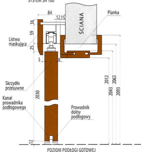
SYSTEM SN 100
