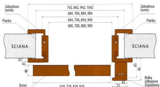
SYSTEM SN100
