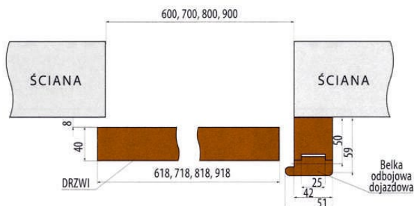
SYSTEM SN 100
